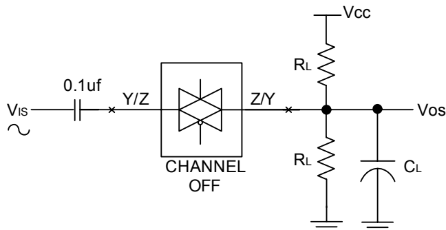
Fig-7 Feed-through Attenuation (Switch OFF)
